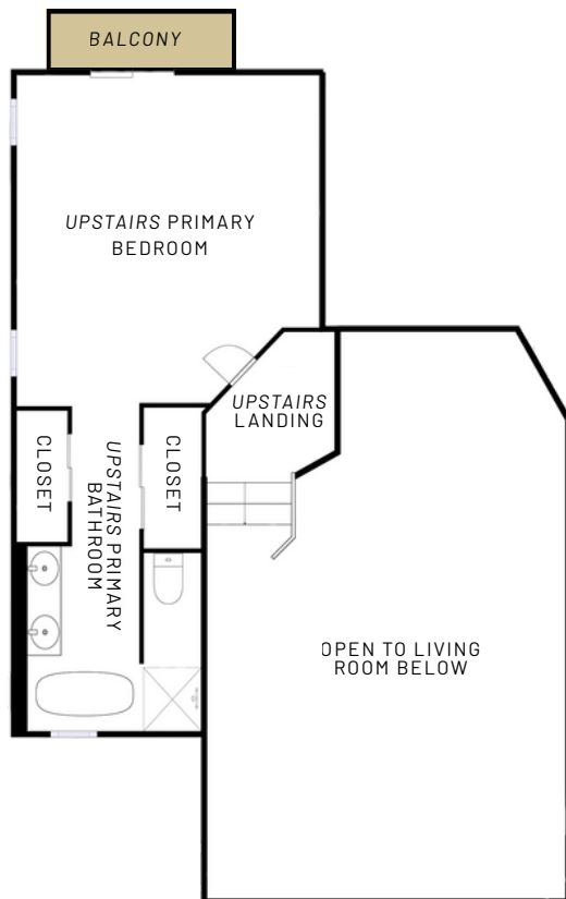
2ND FLOOR
